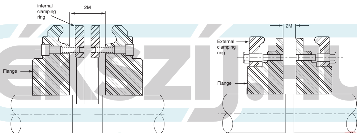
FFX Assembly
